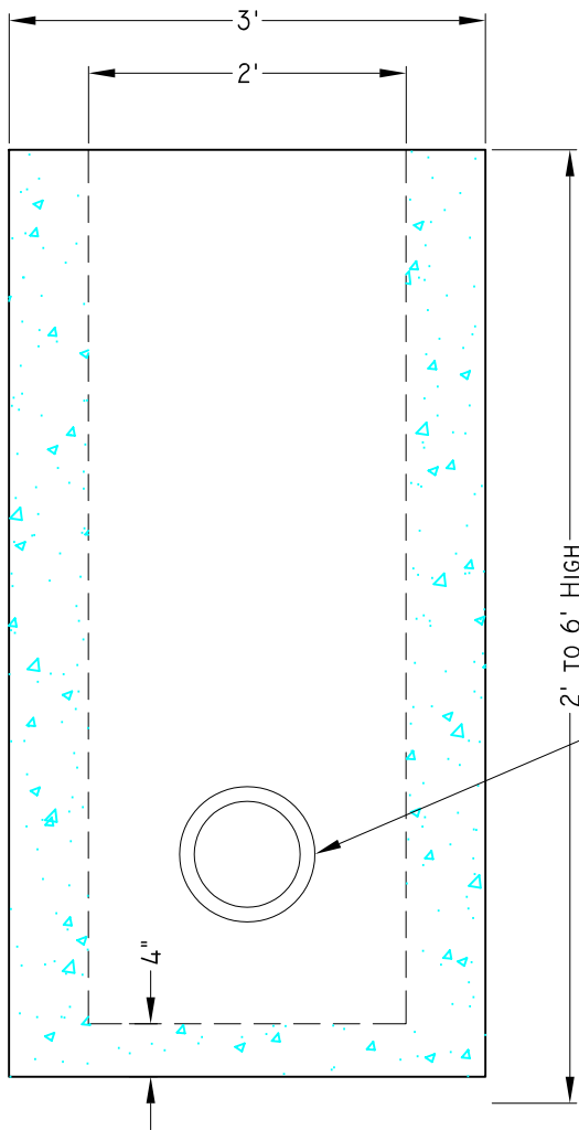
TYPE "F" CATCH BASIN
