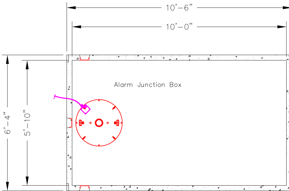
Plan View
