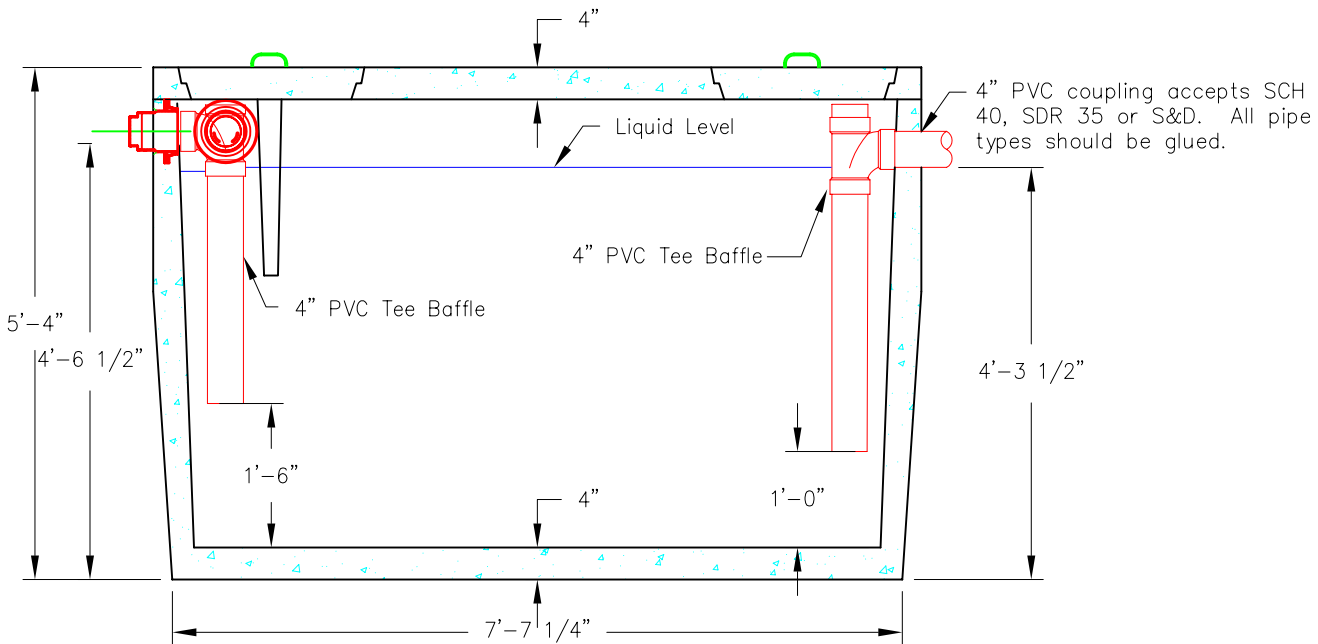
Section View
