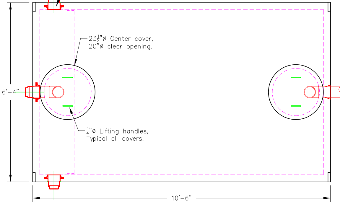
Plan View
