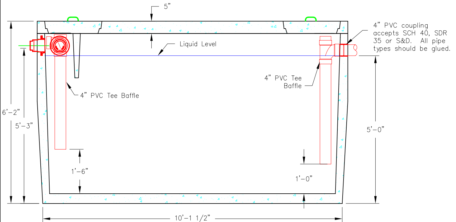
Section View
