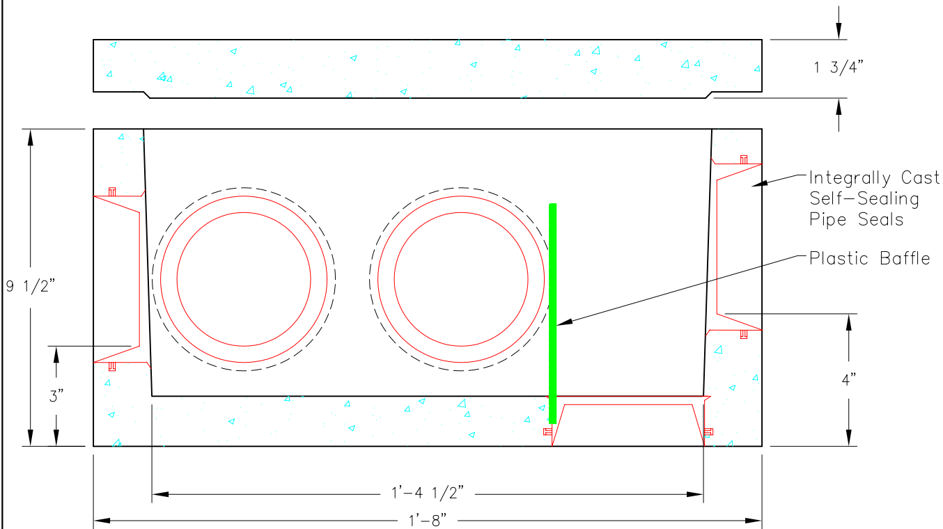
Section View
