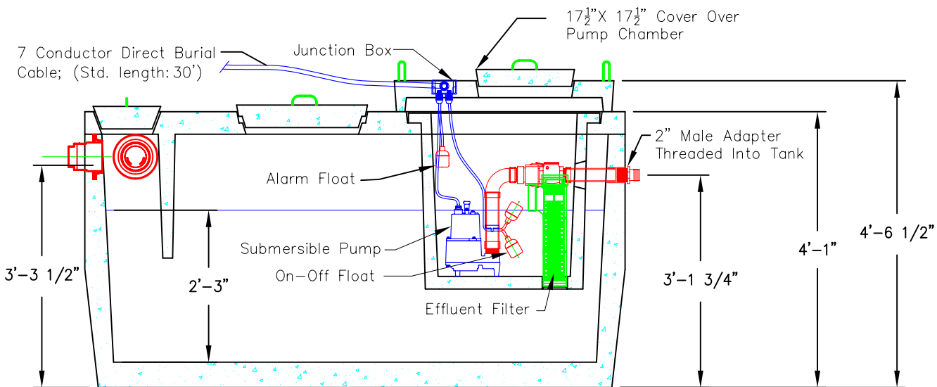
Section View
