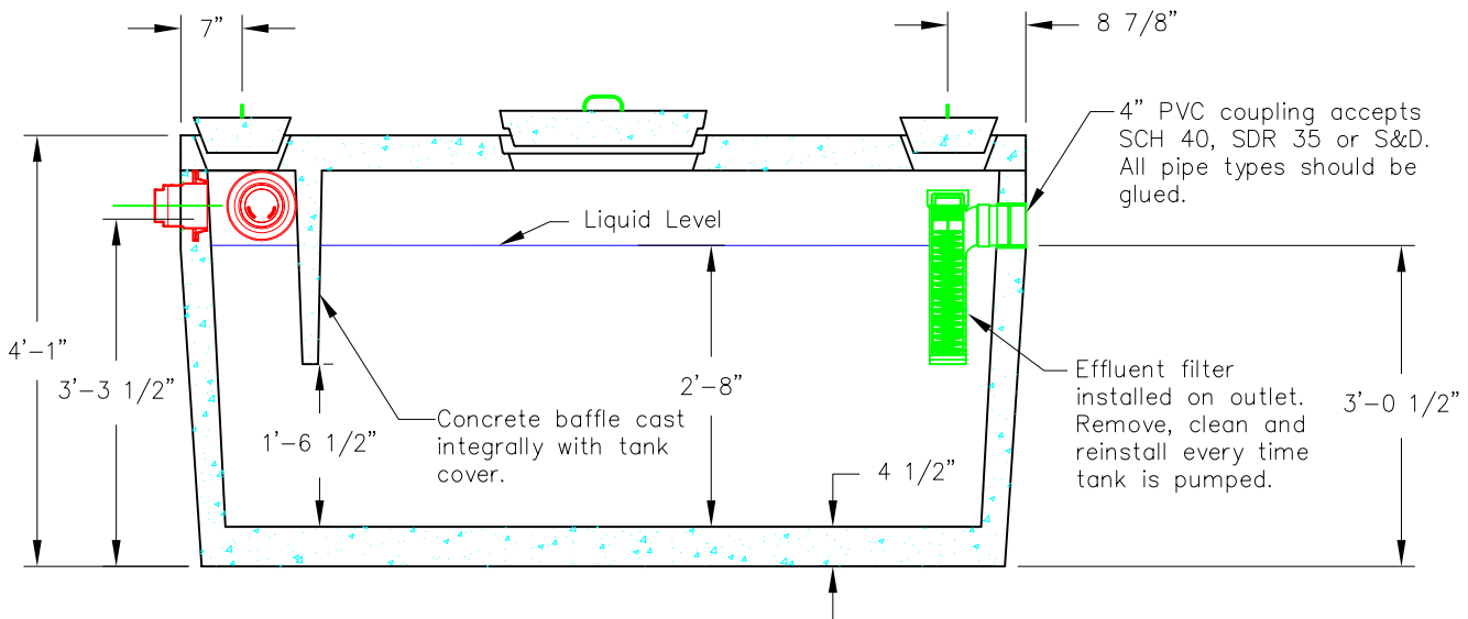
Section View
