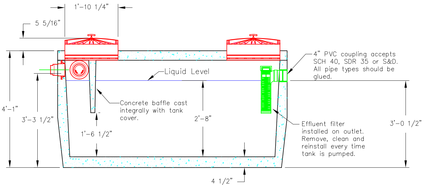
Section View
