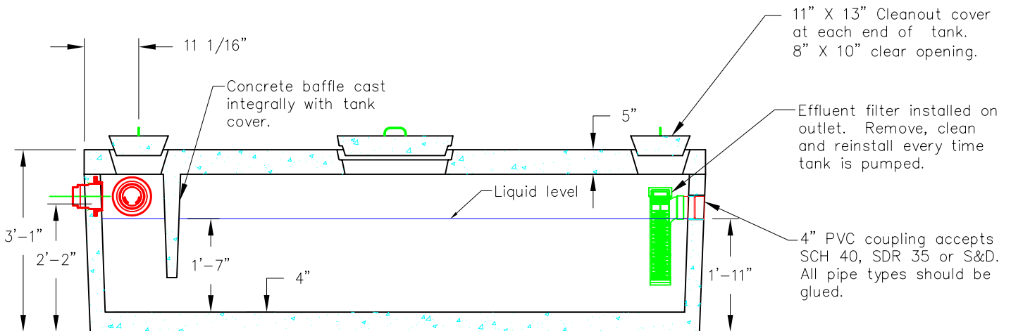
Section View
