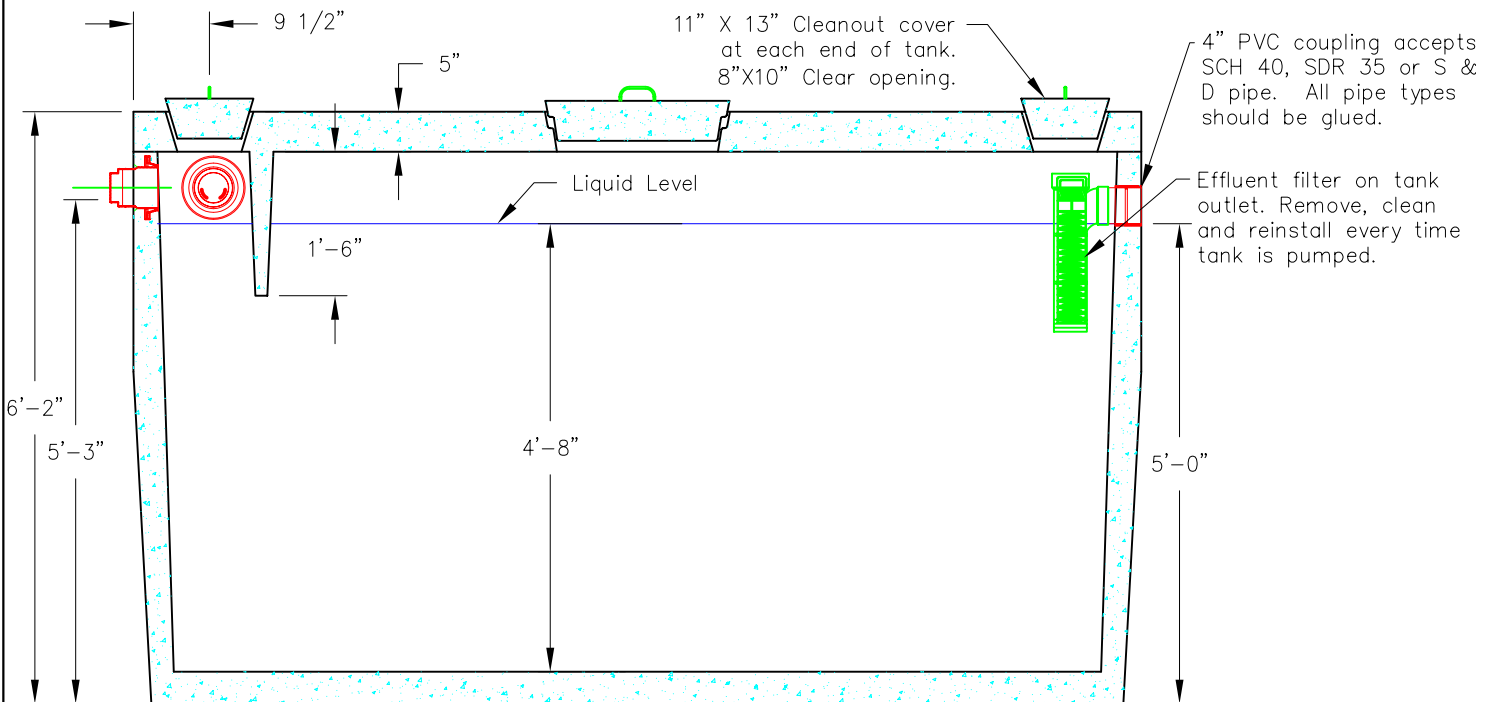
Section View
