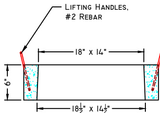
6" SECTION
