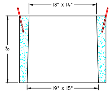
18" SECTION
