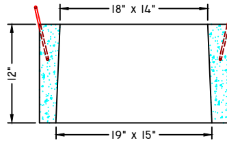
12" SECTION
