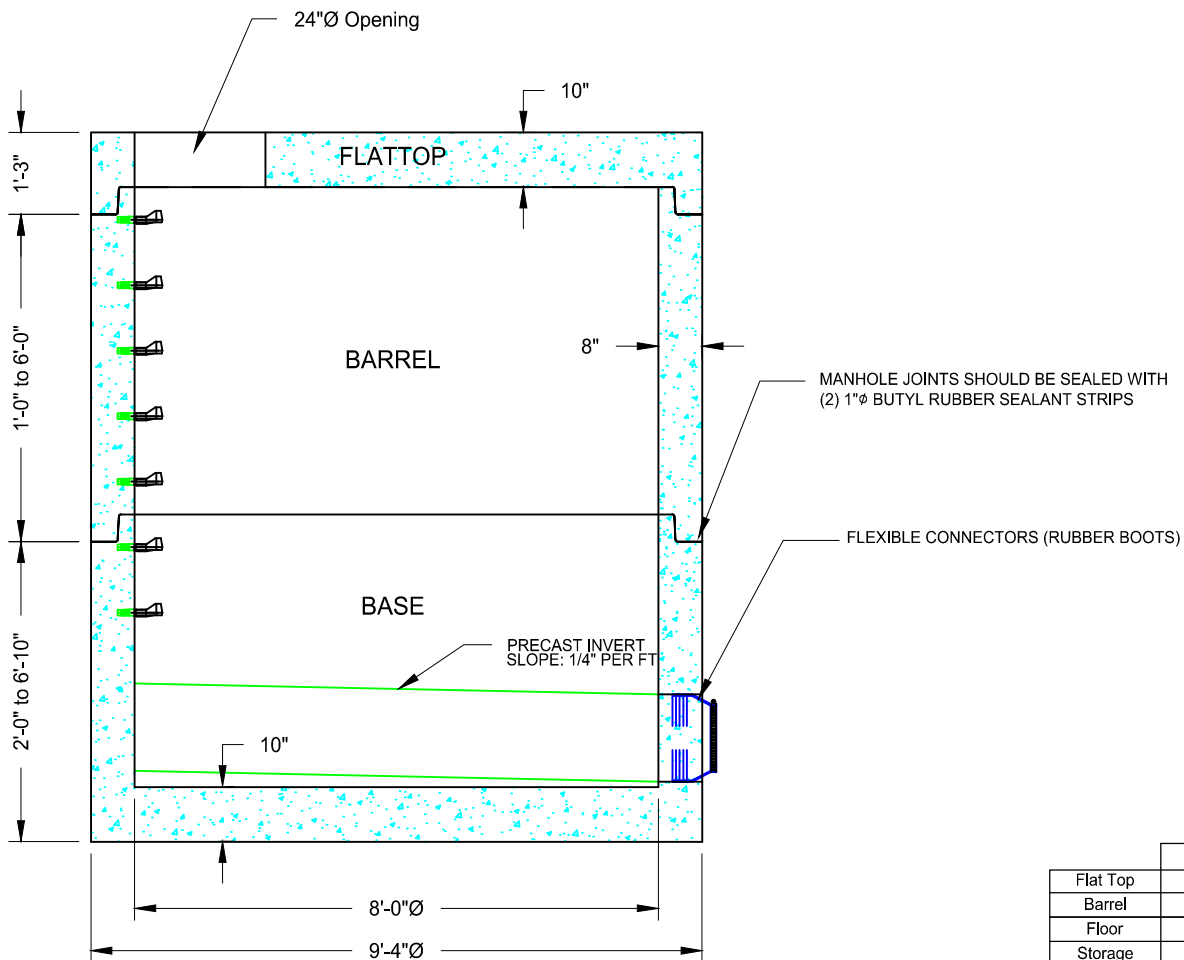
SECTION "A-A"
