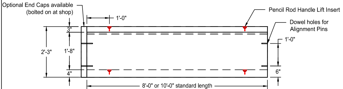
Elevation View
