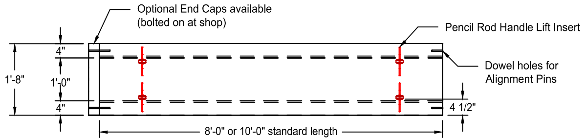
Plan View
