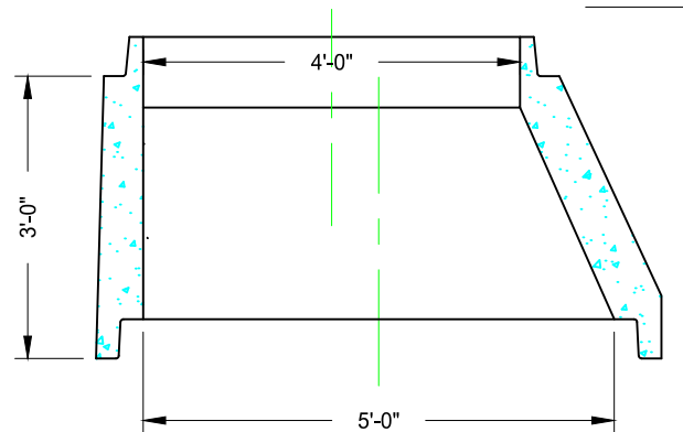
5'x4' TRANSITION CONE
