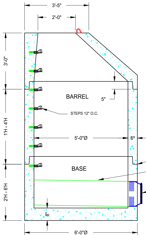
SECTION "A-A"
