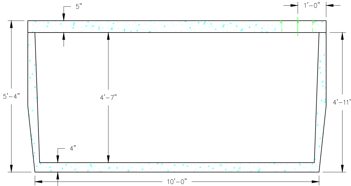
Section View
