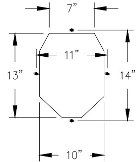
Riser Detail
