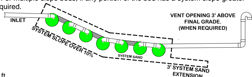
Illustration of bed with multiple slopes:
