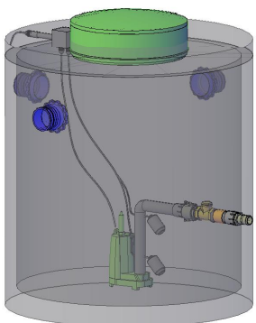
Conceptual View
