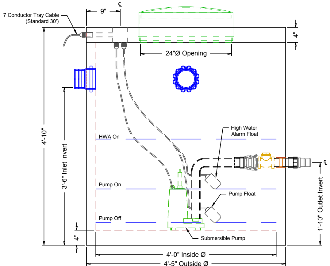
Elevation View
